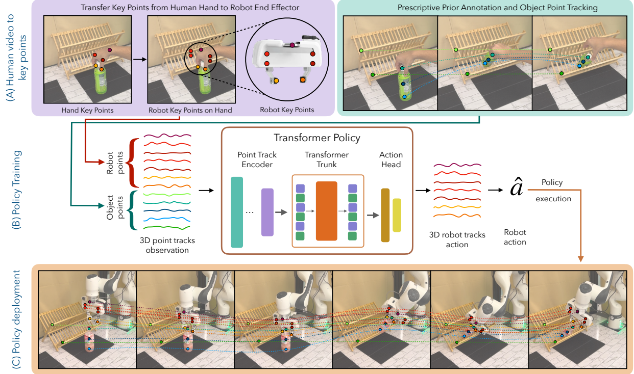
Fig. 3: Overview of the Point Policy framework. (a) Point Policy leverages state-of-the-art vision models and policy architectures to translate human hand poses into robot poses while capturing object states through sparse single-frame annotations. (b) The derived key points are fed into a transformer policy to predict the 3D future point tracks from which the robot actions are computed through rigid-body geometry constraints. (c) Finally, the computed action is executed on the robot using end-effector position control at a 6Hz frequency.
