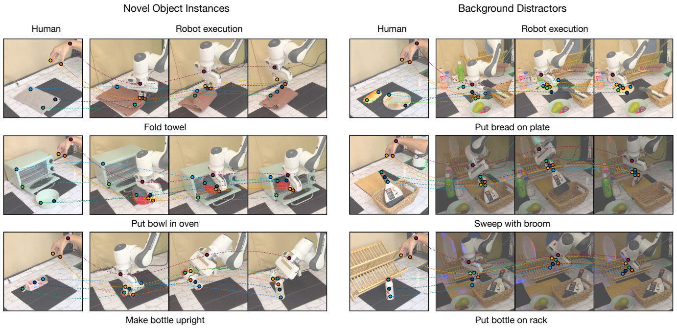
Fig. 6: Real-world rollouts showing that Point Policy generalizes to novel object instances and is robust to background distractors.
