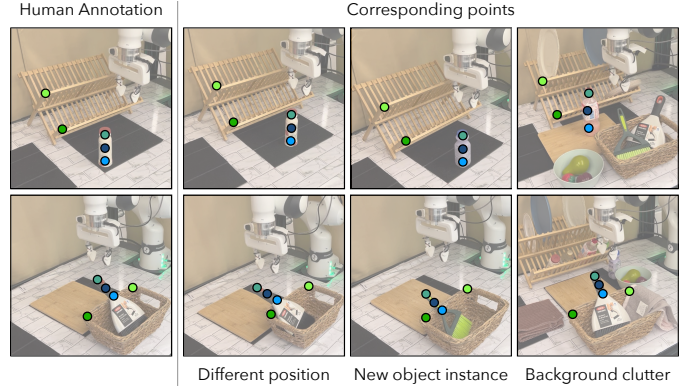
Fig. 4: Results of the correspondence model when used for the put bottle on rack and sweep broom tasks. On the left is a frame with human annotations for the object points. On the right, we show that semantic correspondence can identify the same points across different positions, new object instances, and background clutter.
