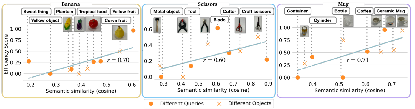
Fig. 21: Generalization plots for unseen queries and objects in the same category: (left) banana , (center) scissors , (right) mug . We see a positive correlation in semantic similarity (cosine distance) of the objects/queries with the most similar object present in our training objects, and the efficiency score suggesting the model's performance.
