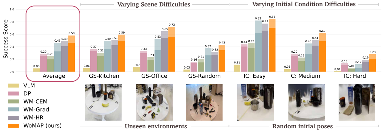
Fig. 5: Gaussian Splat evaluation tasks and results. Success rates (translucent bars) and efficiency scores (solid bars) in active object localization across Gaussian Splat scenes and initial-pose conditions: easy (E), medium (M), and hard (H). As in the PyBullet scenes, WoMAP outperforms all baseline methods via effective action grounding and optimization.
