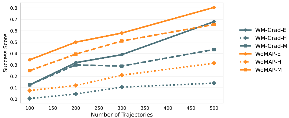
Fig. 18: Average success score for different number of trajectories sampled from 50 scenes in the PB-Kitchen-Easy task. We observe a positive correlation between the number of training trajectories and the success rate of WM-Grad and WoMAP across different initial conditions: Easy (E), Medium (M), and Hard (H). With only 200 training trajectories, WoMAP outperforms the VLM and DP baselines (see Figure 4).
