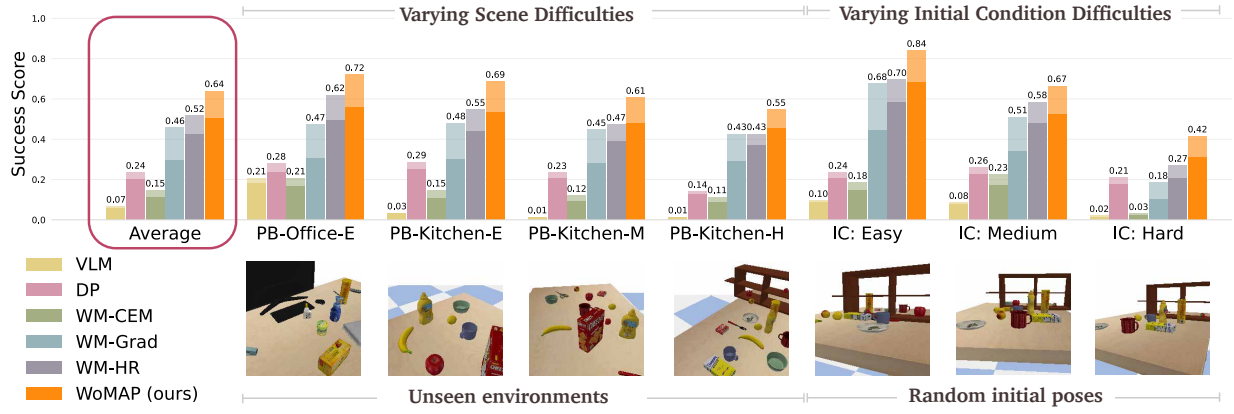
Fig. 4: PyBullet evaluation tasks and results. Success rates (translucent bars) and efficiency scores (solid bars) in active object localization across PyBullet scenes (presented in the order of increasing difficulty) and initial-pose conditions: easy (E), medium (M), and hard (H). WoMAP outperforms all baseline methods in all scenes and initial-pose conditions.
