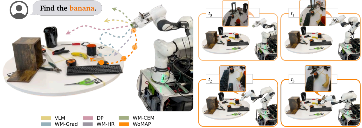
Fig. 3: Visualization of the TidyBot’s trajectories for all planners. When asked to find an object, e.g., a banana occluded by a mug, WoMAP finds the target object (banana) more efficiently than the other planners. As illustrated, the WM-Grad computes inefficient, circuitous paths, while the DP does not look behind occlusions. See Section IV-C and the paper’s video for more details. Further, we show images from the scene and wrist cameras at different timesteps when planning with WoMAP (right).
