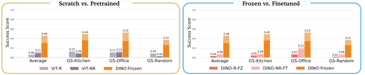
Fig. 11: World Model Architecture Ablations in the Gaussian Splatting Scenes. We ablate training the observation encoder from scratch, finetuning, and training the observation encoder with image reconstruction, where ViT-R denotes a ViT trained from scratch with image reconstruction, ViT-NR denote a ViT trained from scratch without image reconstruction, respectively, DINO-Frozen denotes a frozen DINOv2 encoder, DINO-R-FT denotes a finetuned DINOv2 model trained with image reconstruction, and DINO-NR-FT denotes a finetuned DINOv2 encoder trained without image reconstruction. WoMAP uses DINO-Frozen.
