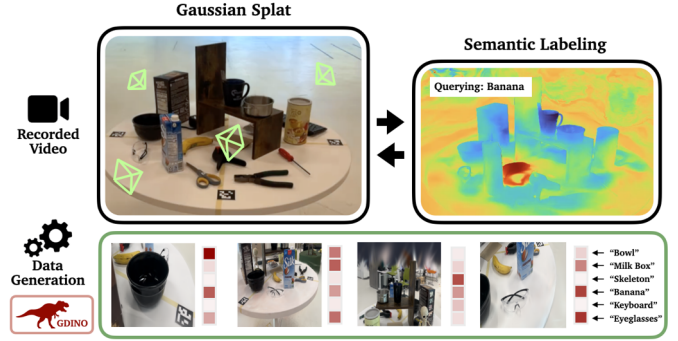
Fig. 6: Data Generation with Gaussian Splats. We train Gaussian Splats for each scene and obtain ground truth object locations through semantic labeling [36] for informative view sampling. Each observation is labeled with GroundingDINO [21] to get confidence scores for all training targets.
